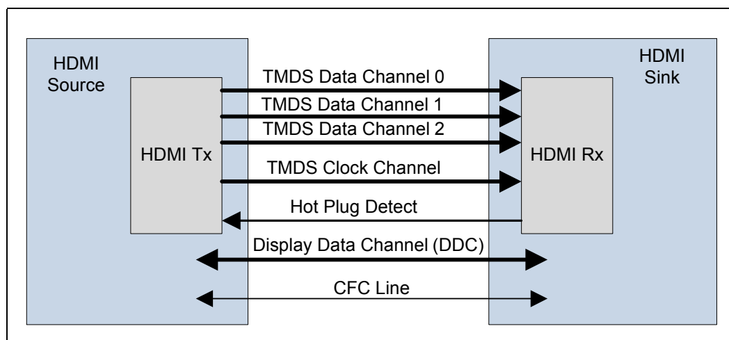
Figure 5-17. HDMI* Overview
