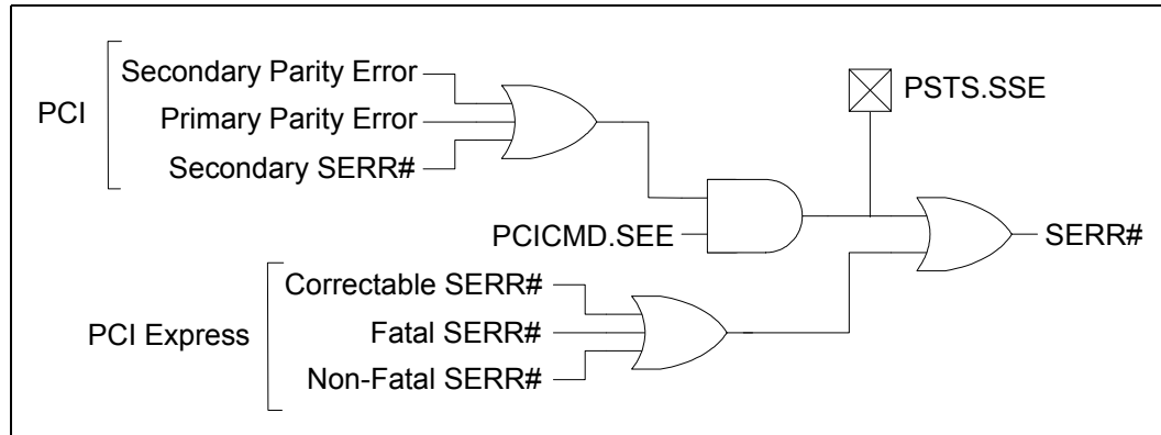
Figure 5-1. Generation of SERR# to Platform
