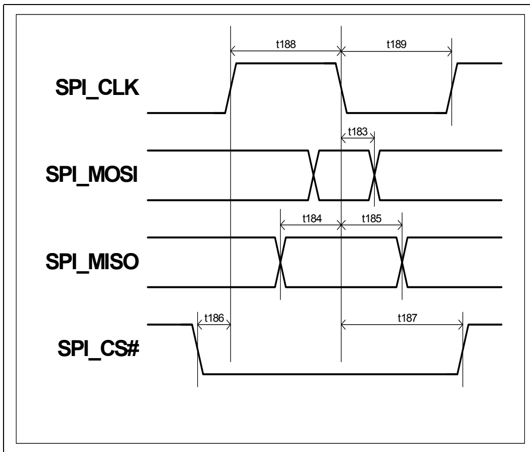
Figure 8-22. SPI Timings
