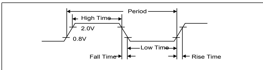
Figure 8-11. Clock Timing
