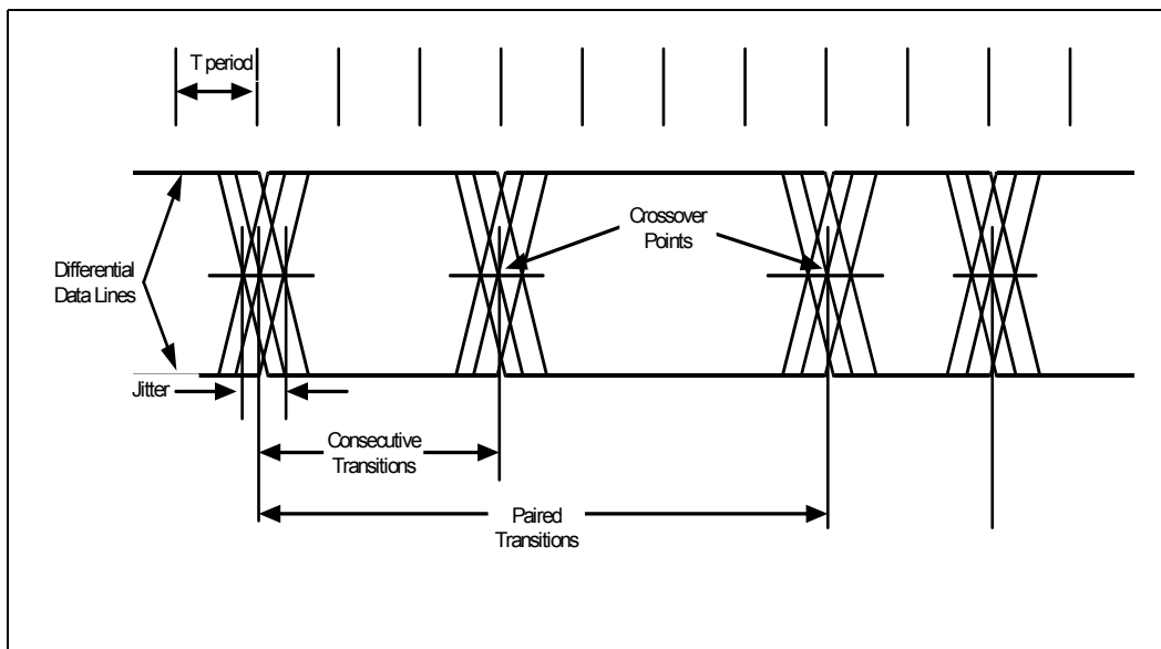
Figure 8-18. USB Jitter
